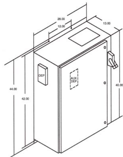
"ML" Enclosure
